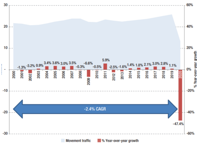
Chart 68: Evolution of annual aircraft movements in Europe (2000–2020)
